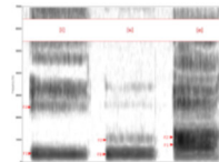
Spectrogram of American English vowels [i, u, o] showing the formants f 1 and f 2
